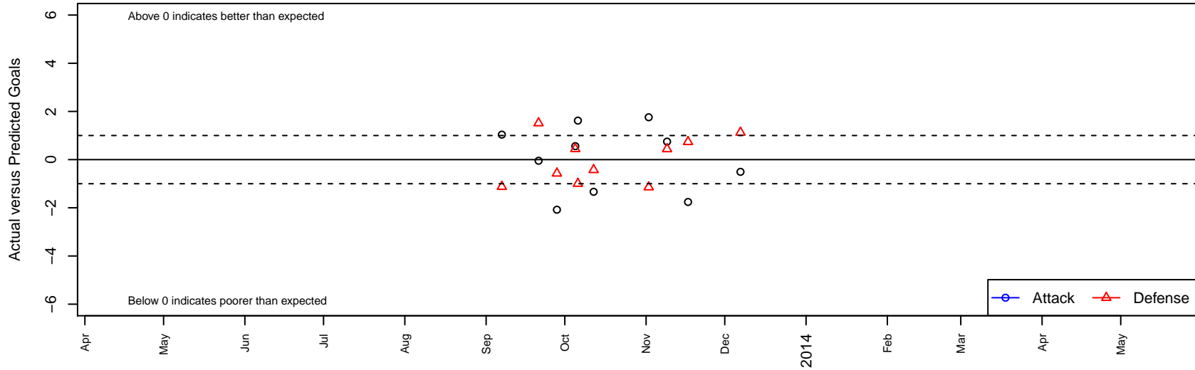
PSA Storm Black B00 Dots are actual minus expected GF (blue circles) and GA (red triangles). Blue line is smoothed change in attack strength. Red is smoothed change in defense strength.
